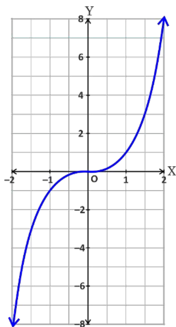
Graph of f(x) = x^3
